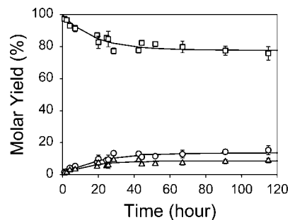
FIGURE 5. Mole fraction product yields as a function of time for the reaction of phenol with tert -butyl alcohol in water at 250 °C and 172 bar: phenol ( \square ); 2- tert -butylphenol ( \circ ); 4- tert -butylphenol ( \triangle ). 16
